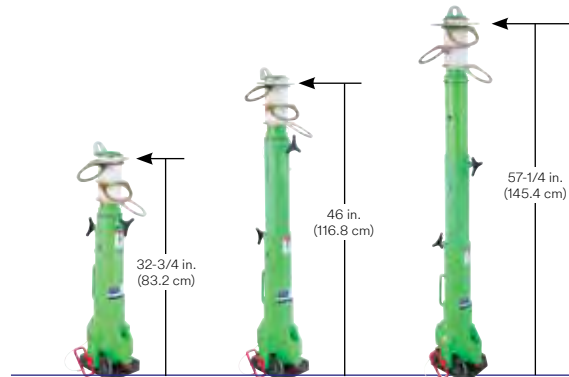
Telescoping design: Overall height can be adjusted from 32-3/4 in.-57-1/4 in. (83.2 cm-145.4 cm)
